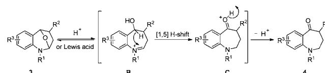
Scheme 2. Potential Cascade Reactions of C–O Bond Cleavage/1,5-Hydride Transfer From Benzazepine 3 to Benzazepinone 4
