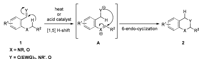
Scheme 1. Typical Internal Redox Process
